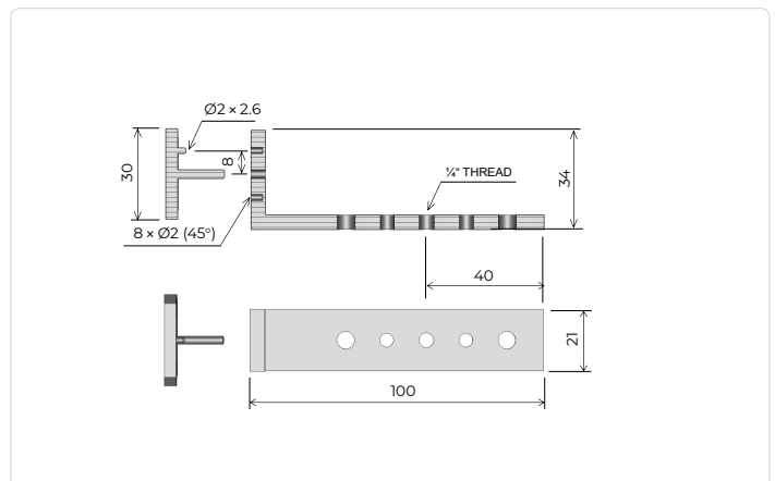
Mounting flange
